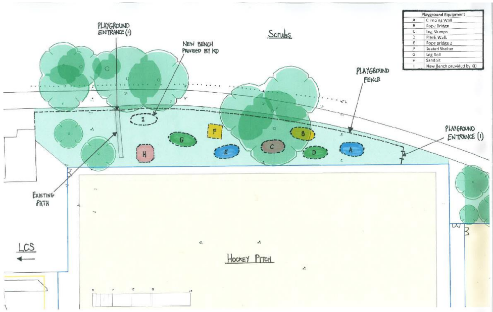
Playground Layout Scale 1:300
